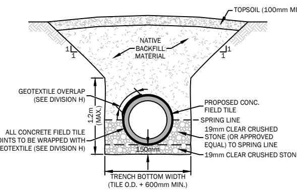
TYPICAL CONCRETE TILE INSTALLATION ON STONE BEDDING DETAIL (PROVISIONAL ITEM) N.T.S.
