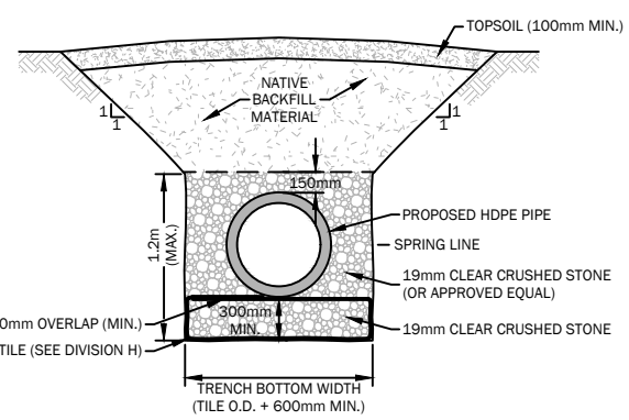
TYPICAL HDPE PIPE INSTALLATION ON WRAPPED STONE BEDDING DETAIL (PROVISIONAL ITEM) N.T.S.
