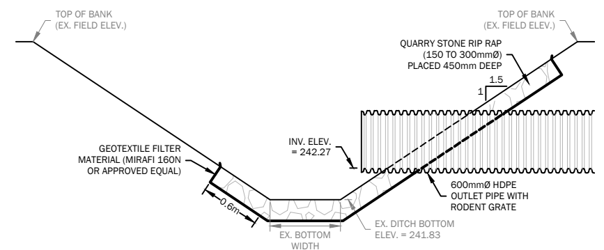
TYPICAL OUTLET DETAIL N.T.S.
