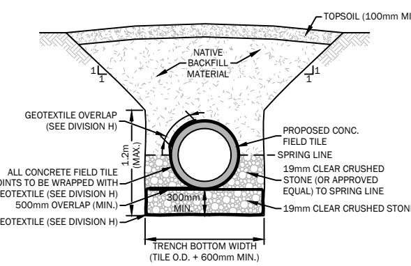
TYPICAL CONC. TILE INSTALLATION ON WRAPPED STONE BEDDING DETAIL (PROVISIONAL ITEM) N.T.S.
