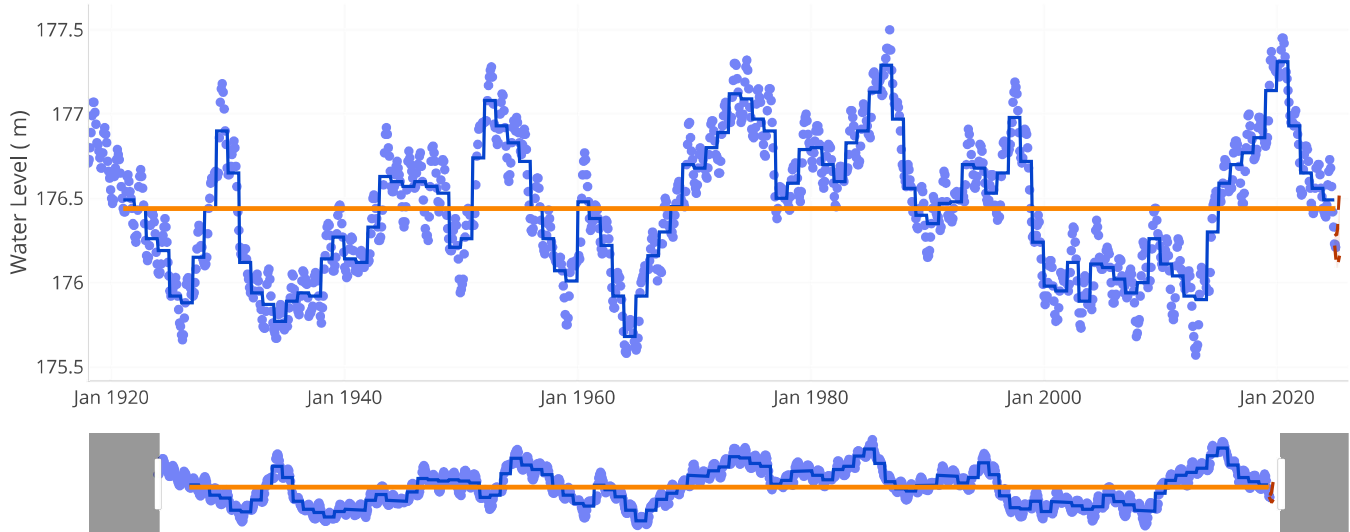
Lakes Michigan and Huron Water Levels
