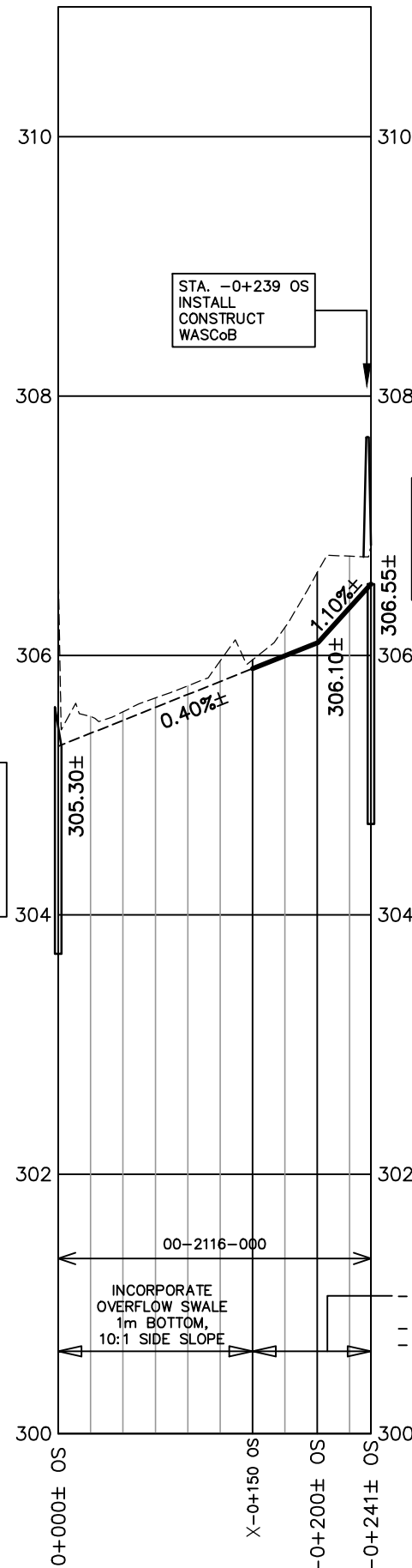
PROFILE - OVERFLOW SWALE
