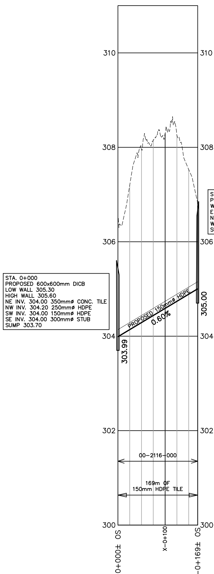
PROFILE - TILE
