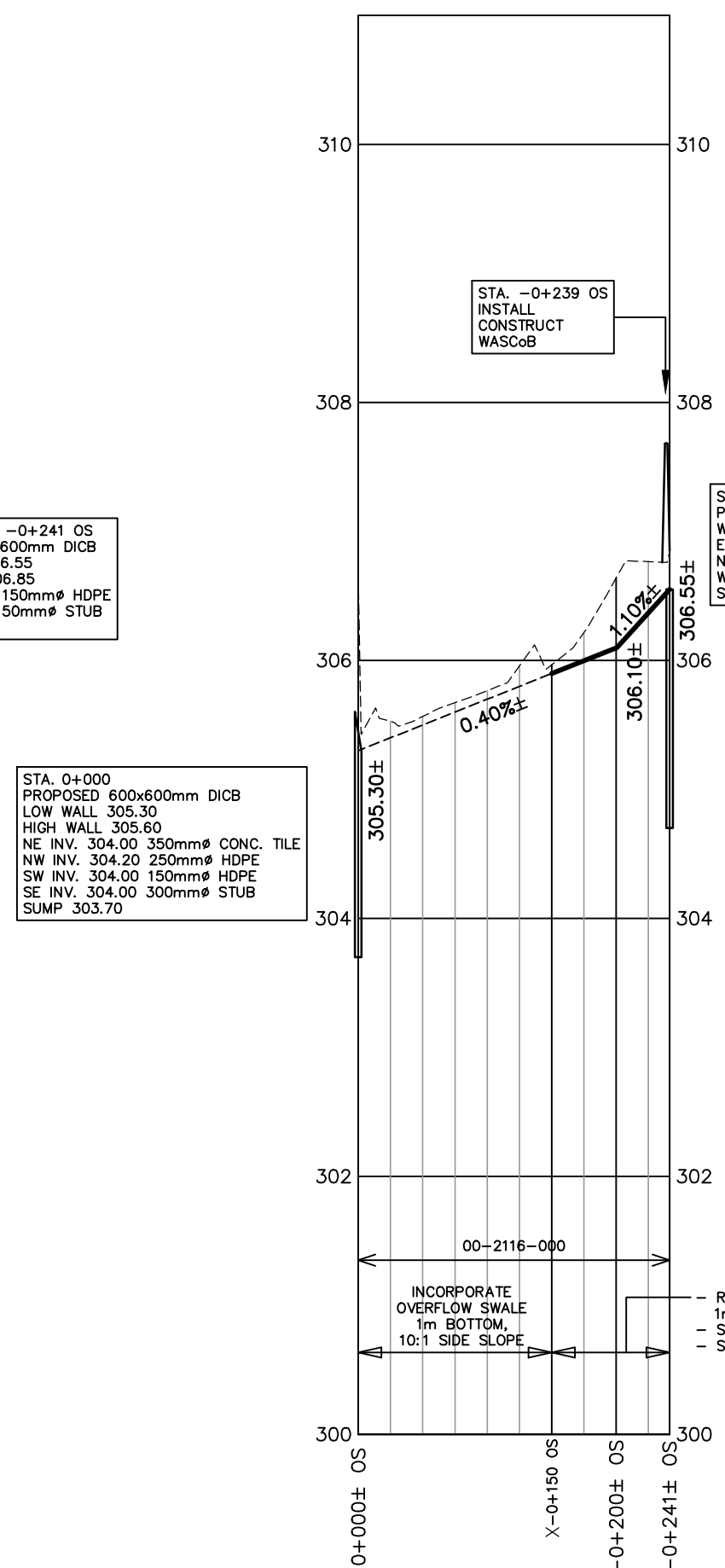
PROFILE - OVERFLOW SWALE
