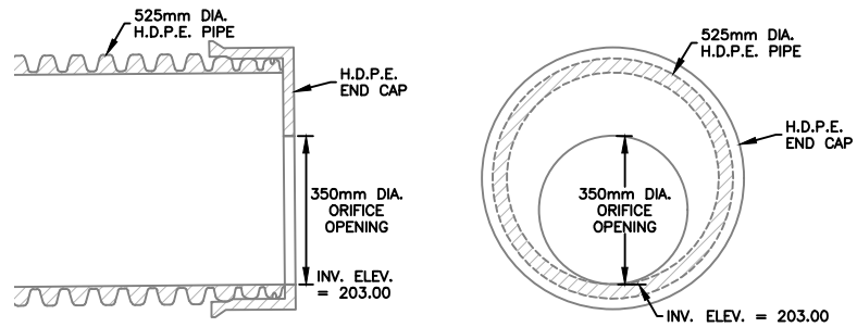
ORIFICE END CAP DETAIL
