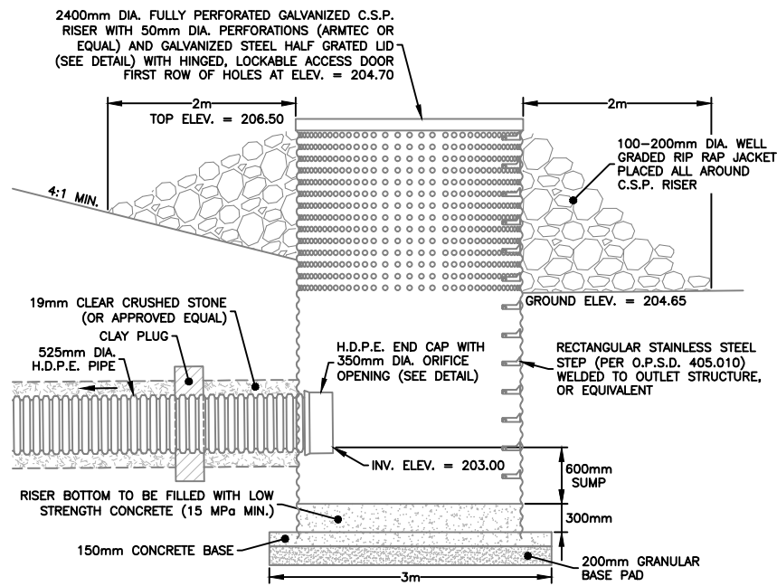
RISER PIPE OUTLET DETAIL
